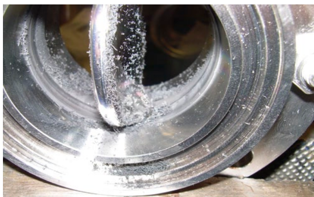
Figure 1. Seal abrasion at the disc.
